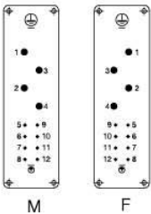
接插针排序 Contacts arrangement view from termination side
