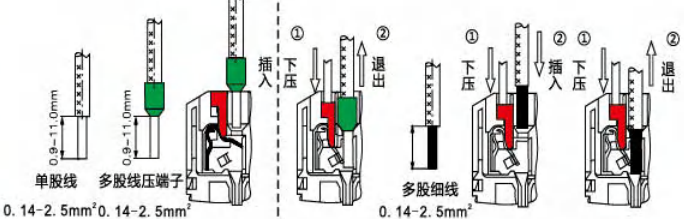
Step 2:接线完成 Connection completion
