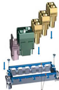
装配前松开滑动边框 Loosen sliding border before assembly
