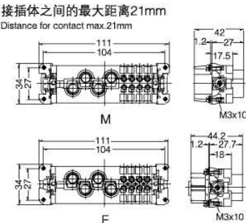
接插针排序 Contacts arrangement view from termination side
